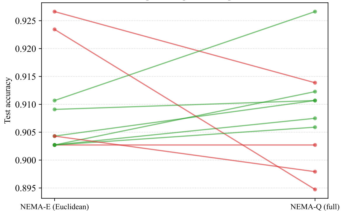
disease: per-seed paired comparison
