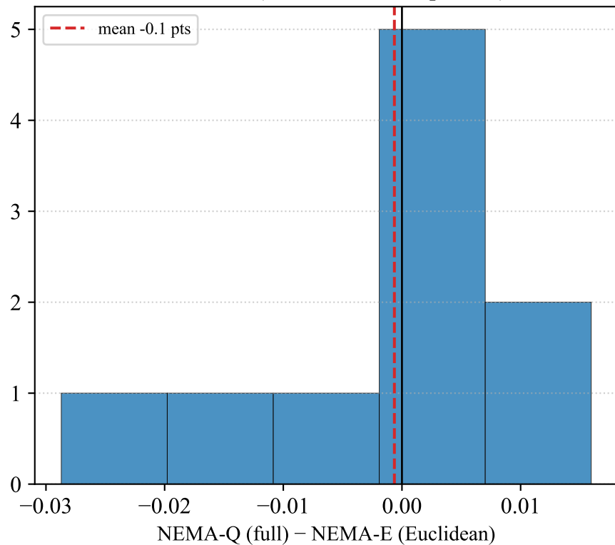
Paired diff (n=10, Wilcoxon p=0.91)
