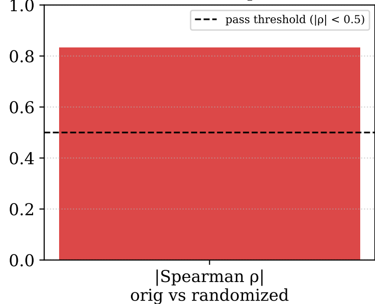
(c) Randomization — passes: False
