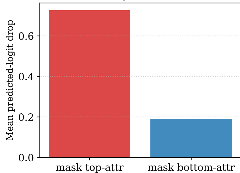
(a) Masking — faithful: True
