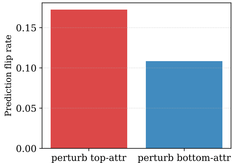
(b) Perturbation — faithful: True
