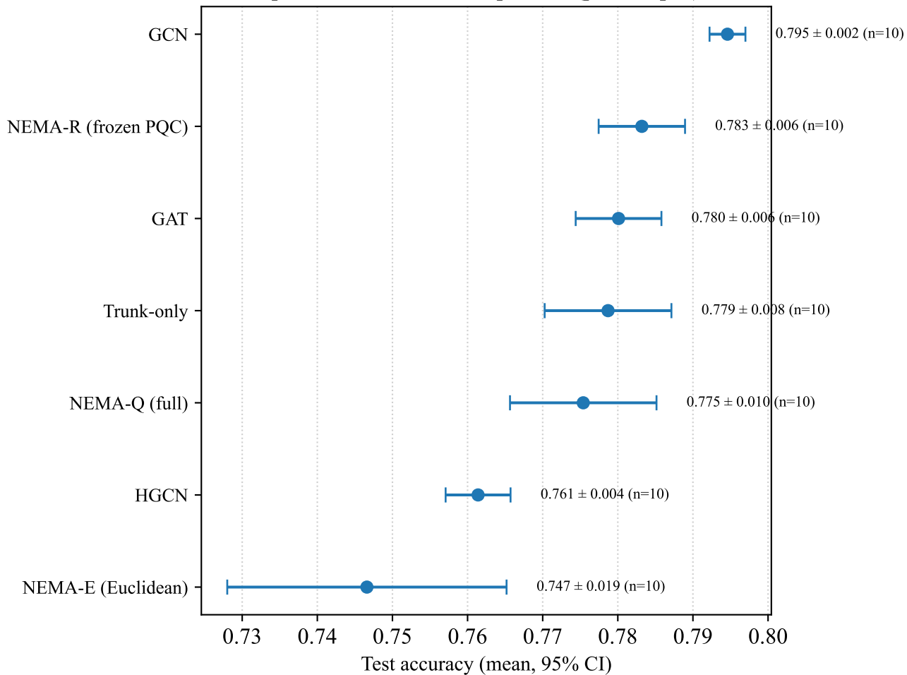
pubmed — model comparison (public split)
