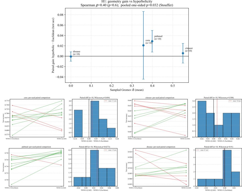
Fig. 6 Geometry \times \delta . Top: paired hyperbolic–Euclidean gain (mean \pm 95% CI) against dataset \delta_{\text{mean}} ; the preregistered H1(b) prediction is a negative slope, the observed trend is positive. The in-panel pooled annotation uses paired t -tests (descriptive); the registered pooled statistic (Stouffer over one-sided Wilcoxon tests, p = 0.040 ) is reported in the text. Bottom: per-dataset paired-seed plots (NEMA-Q vs. NEMA-E).
