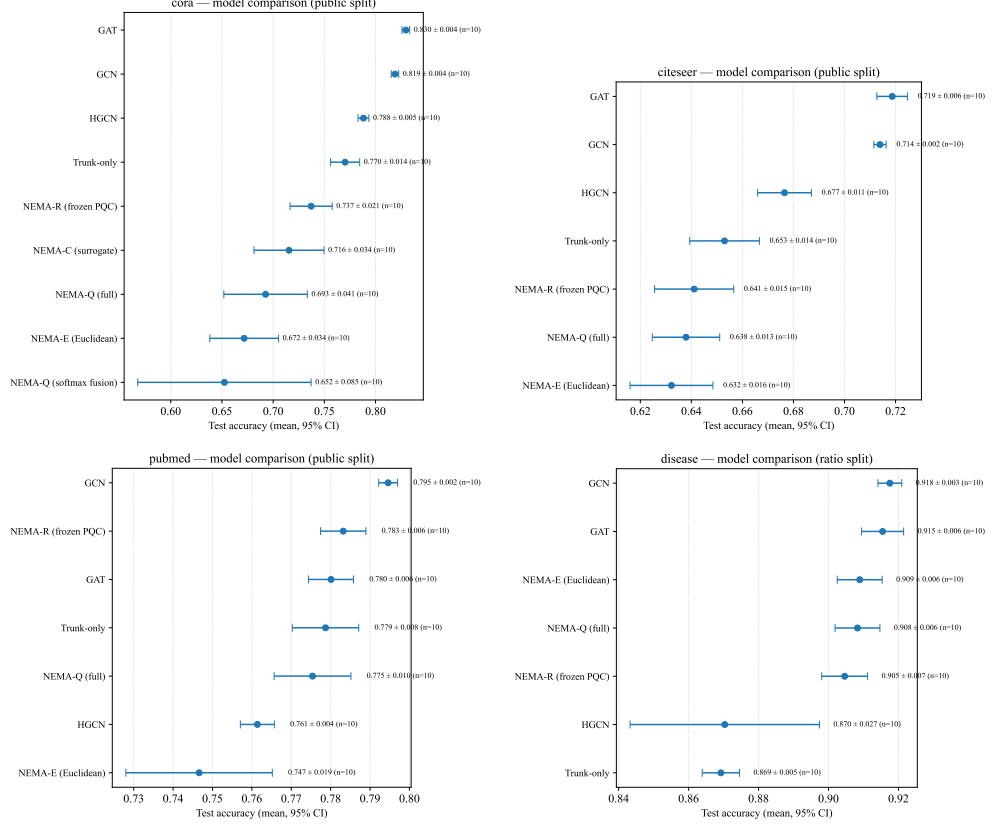
Fig. 3 Forest plots, one panel per dataset: test accuracy (mean ± 95% CI over 10 paired confirmatory seeds) for all baselines, NEMA-Q, and every configuration-swap control under that dataset’s locked recipe.
