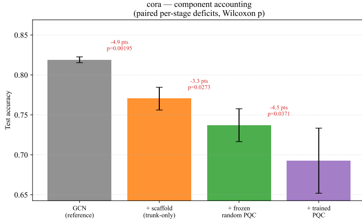
Fig. 2 Component-accounting waterfall on Cora (confirmatory). Each bar is a configuration swap from the previous one; annotations give the paired step size and Wilcoxon p . The decomposition sums exactly to the GCN→NEMA-Q deficit.
