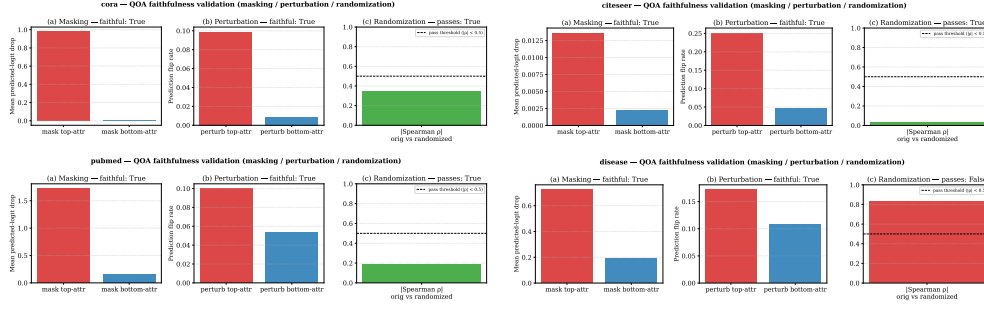
Fig. 7 QOA faithfulness harness, one panel per dataset (pilot models): masking logit-drops (top vs. bottom observable), perturbation flip rates (top vs. bottom), and the randomization Spearman \rho against its 0.5 threshold. Disease fails the randomization check only.
