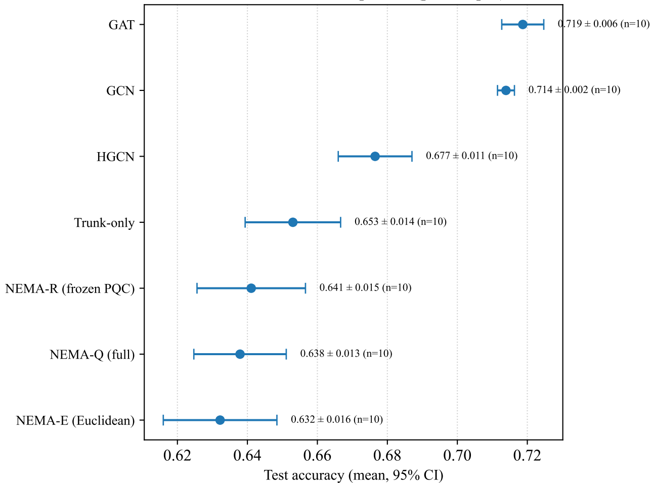
citeseer — model comparison (public split)
