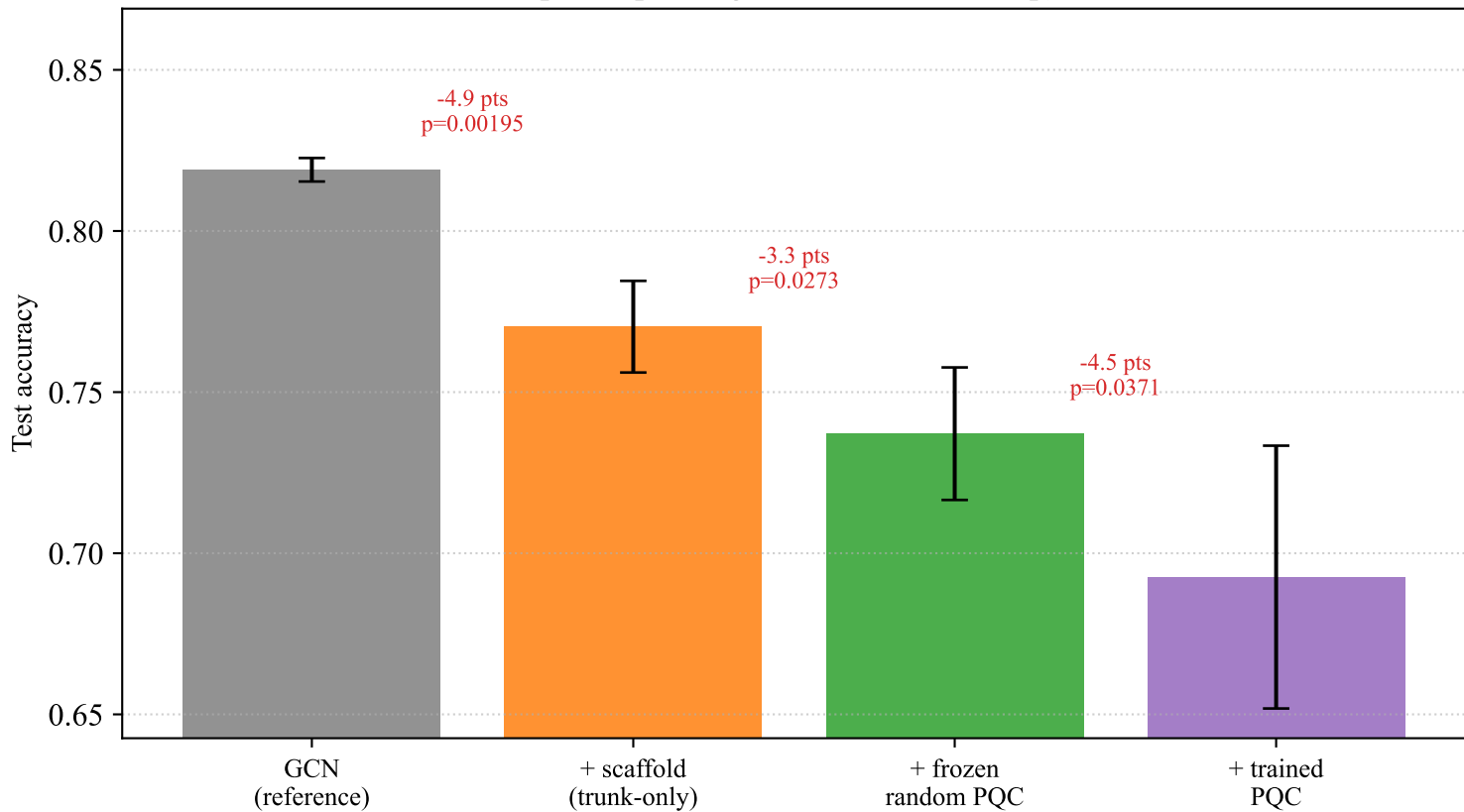
cora — component accounting (paired per-stage deficits, Wilcoxon p)
