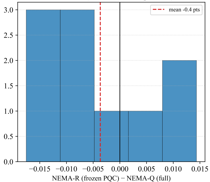
Paired diff (n=10, Wilcoxon p=0.369)
