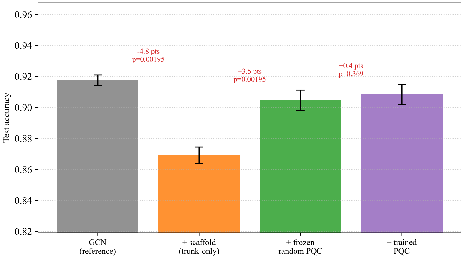
disease — component accounting (paired per-stage deficits, Wilcoxon p)
