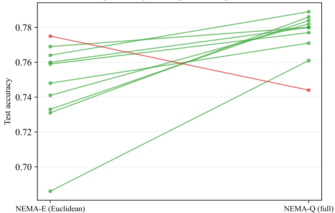
pubmed: per-seed paired comparison
