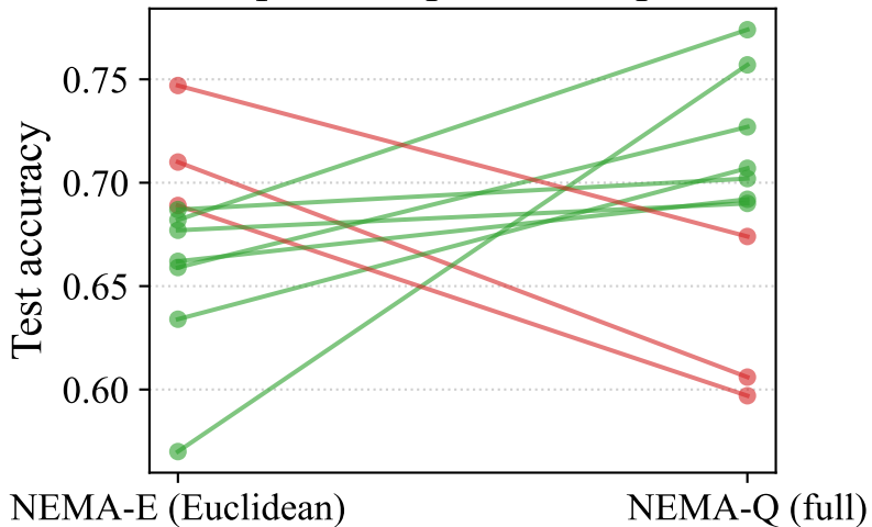
cora: per-seed paired comparison
