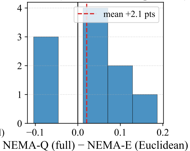
Paired diff (n=10, Wilcoxon p=0.604)
