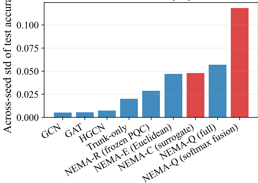
cora — seed stability by model
