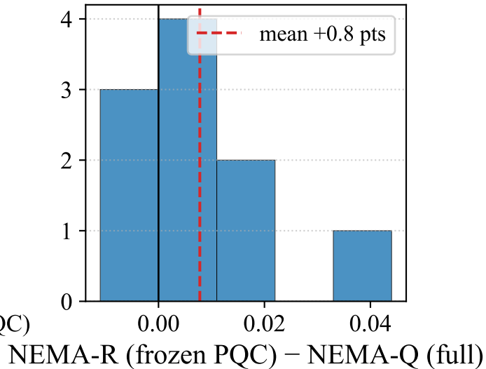
Paired diff (n=10, Wilcoxon p=0.338)
