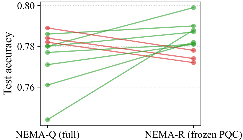
pubmed: per-seed paired comparison
