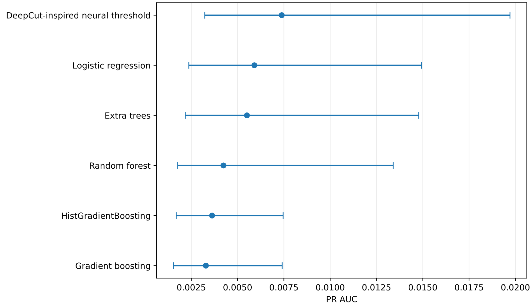
Firm-clustered 95% CIs for PR-AUC
