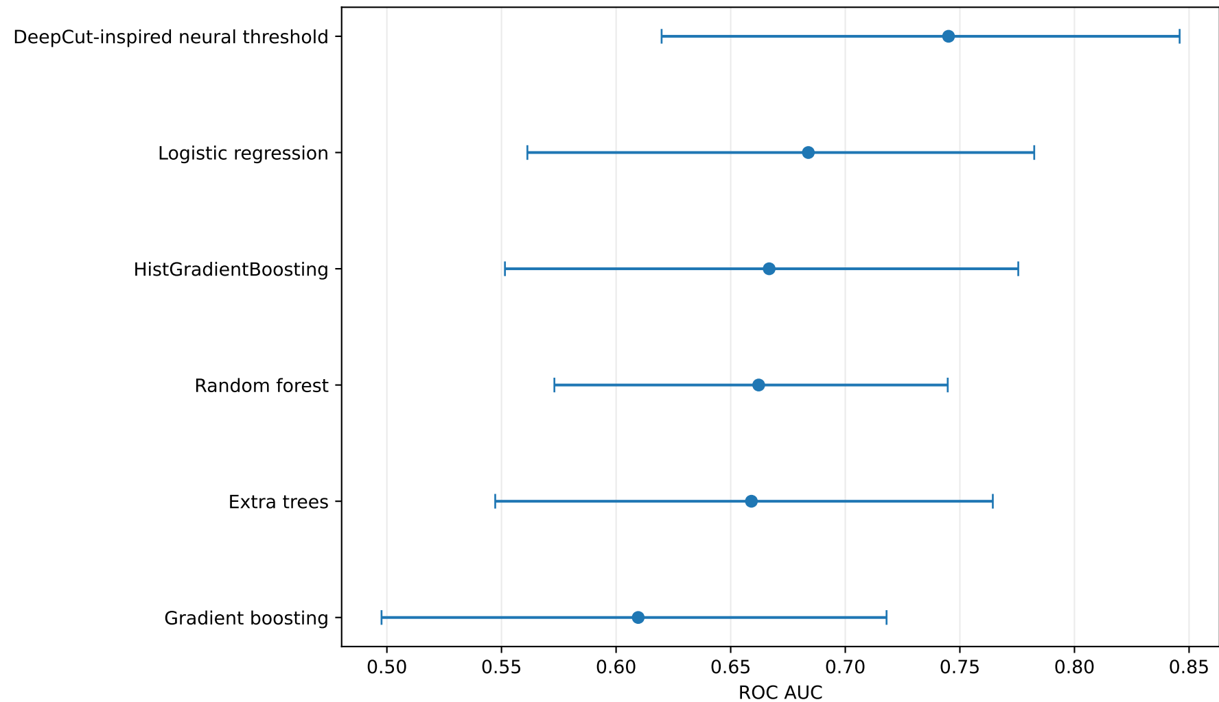
Mature FY2021-FY2022 firm-clustered ROC-AUC intervals
