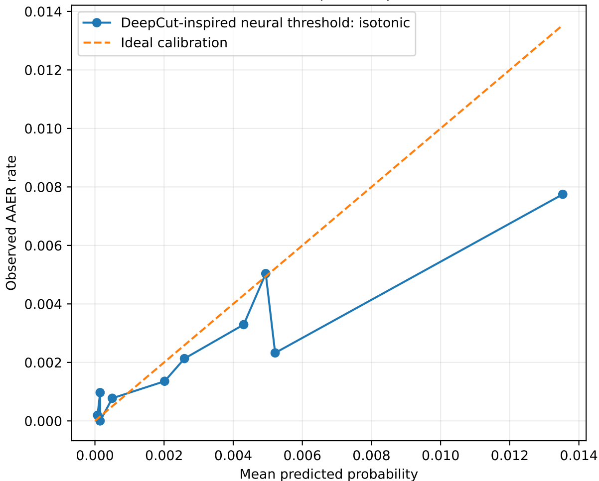
Mature-test calibration: DeepCut-inspired neural threshold
