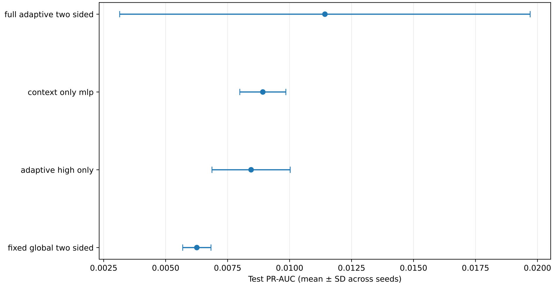
DeepCut repeated-seed stability and structural ablations
