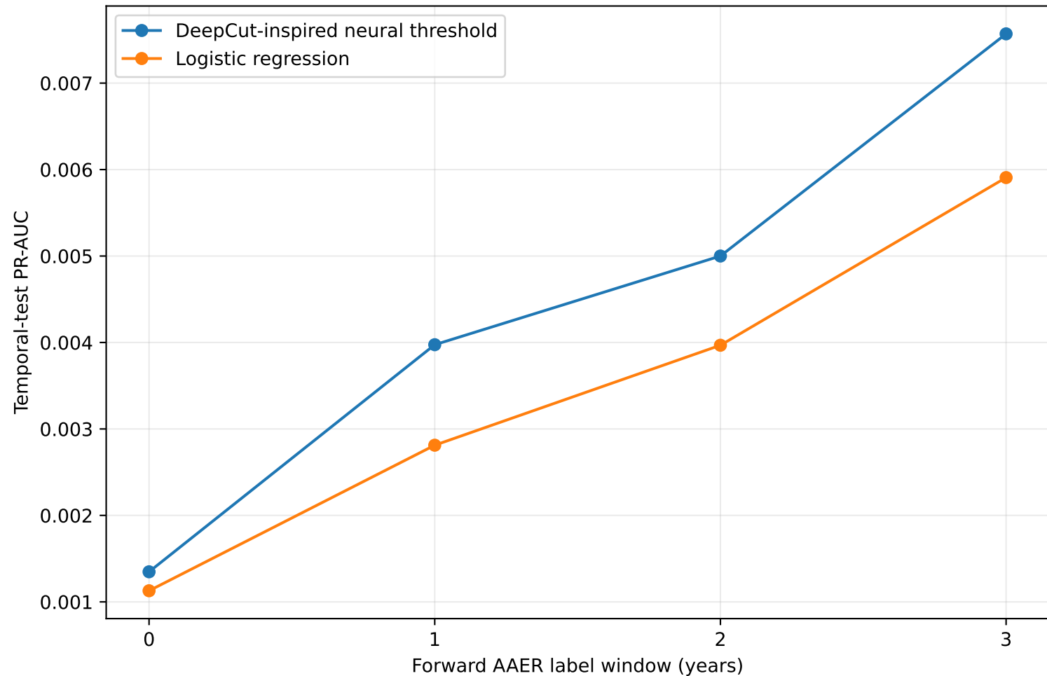
Sensitivity to AAER labeling window
