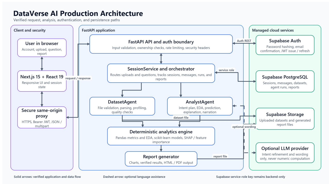
Figure 19: Architecture Diagram
