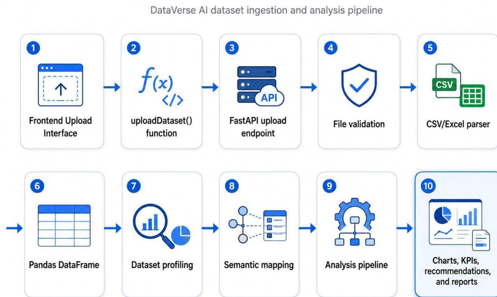
Figure 6.1: Dataset Upload Workflow
