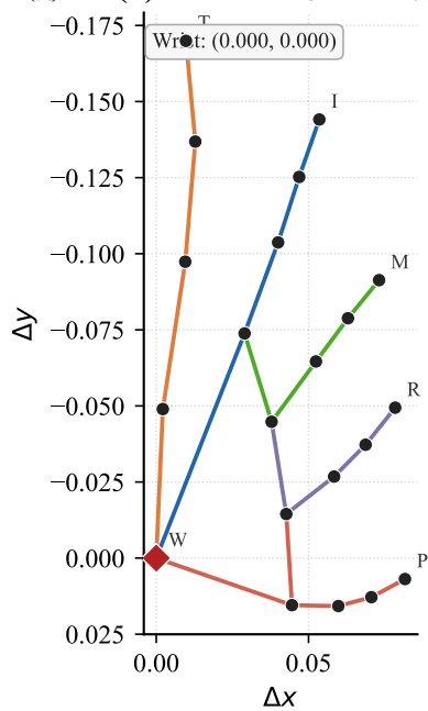
(b) After Wrist-Centered Normalization
