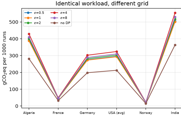
Fig. 3. Emissions of 1000 UCI-HAR runs across six grid carbon intensities. The gap between private and non-private curves is the carbon attributable to privacy.
