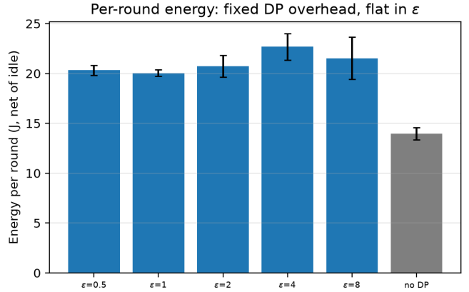
Fig. 2. Net energy per round on UCI-HAR by privacy budget, mean \pm 1 SD over three seeds; the non-private baseline is in grey.
