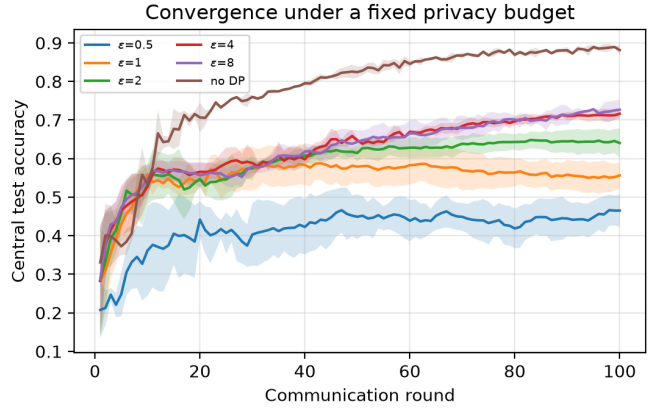
Fig. 1. Central test accuracy per round on UCI-HAR, mean \pm 1 SD over three seeds. No stopping round is marked: on HAR no peak-to-final drop clears the across-seed spread.
