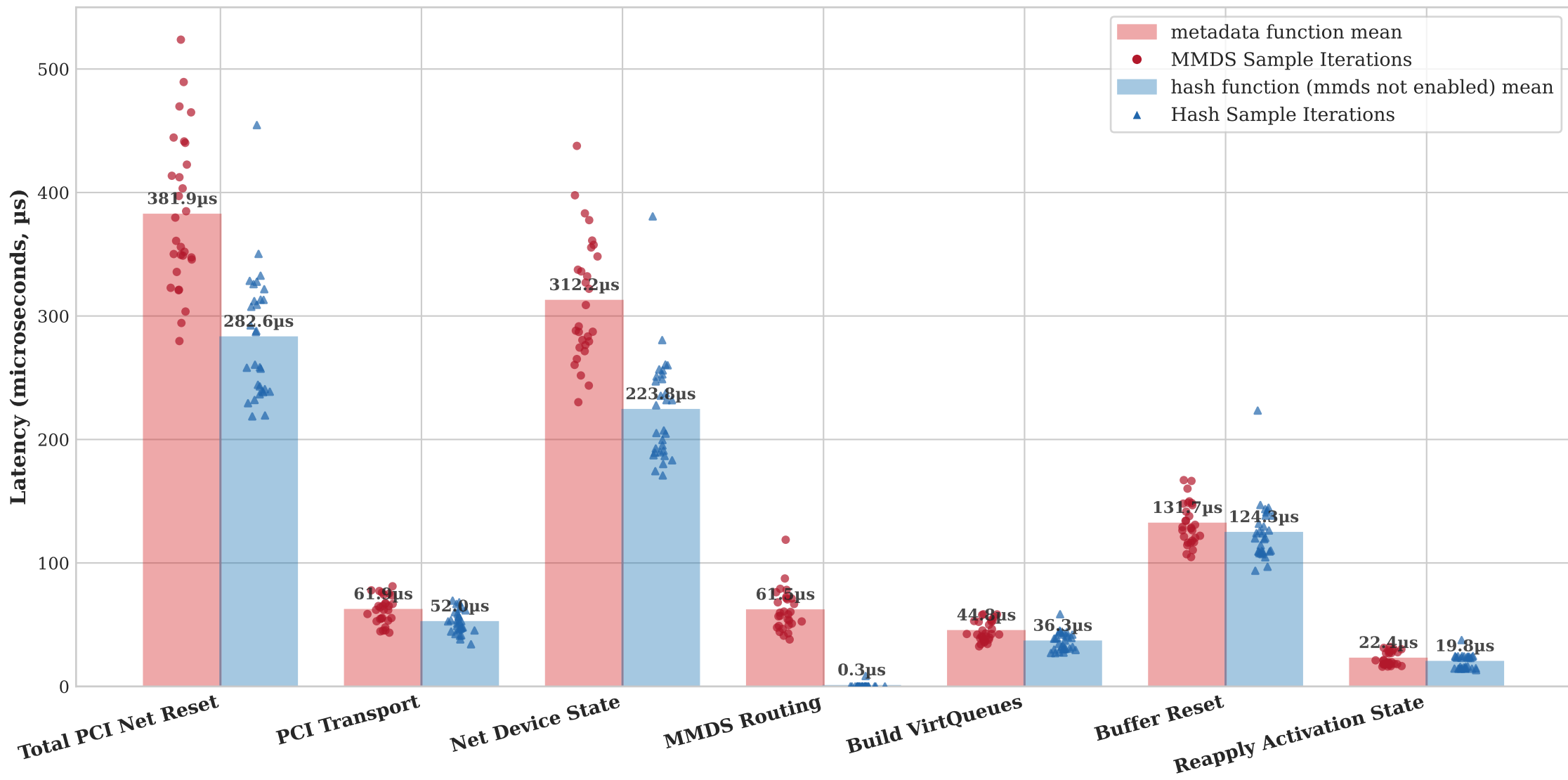
Network Reset Latency Comparison: Active MMDS Subsystem vs. Hash Control Baseline
