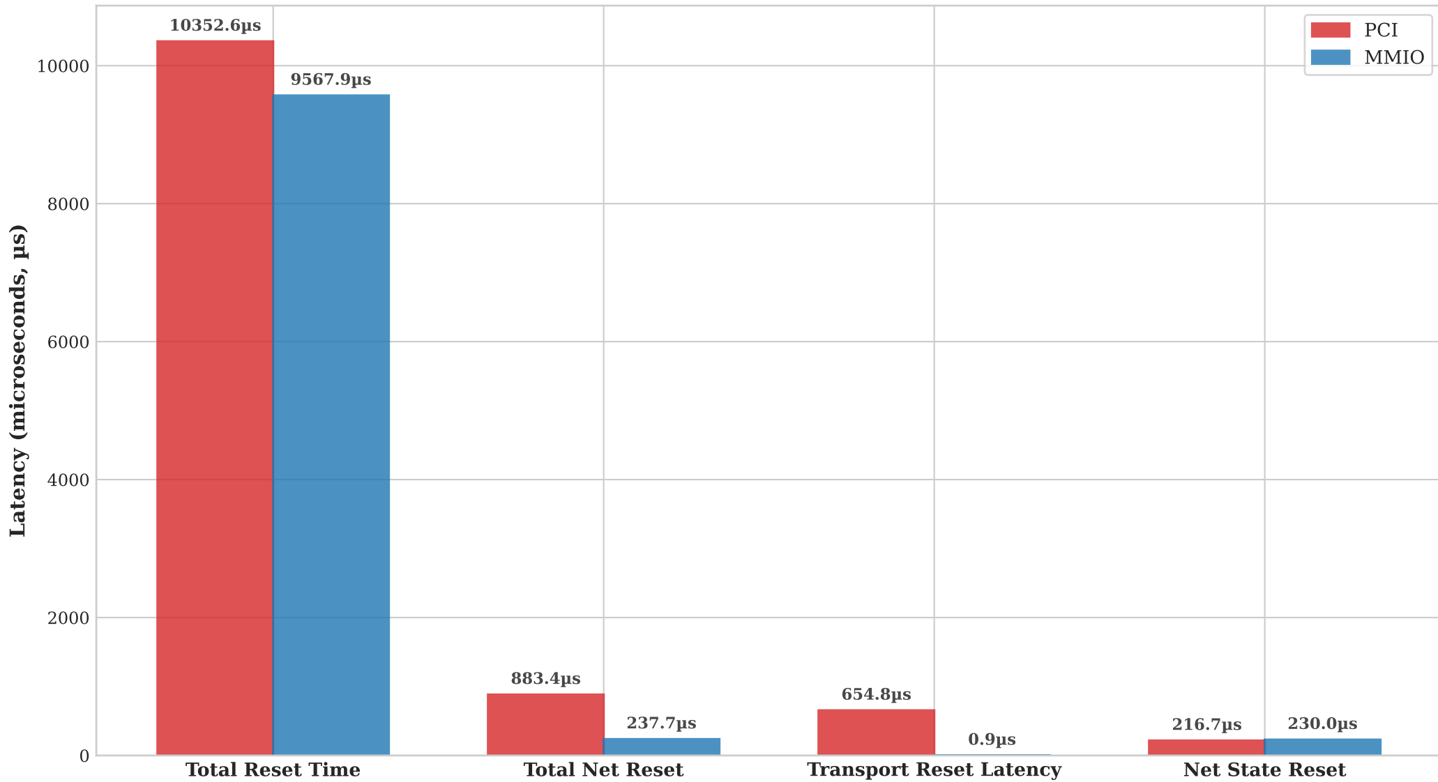
Latency Profiles: PCI vs. MMIO
