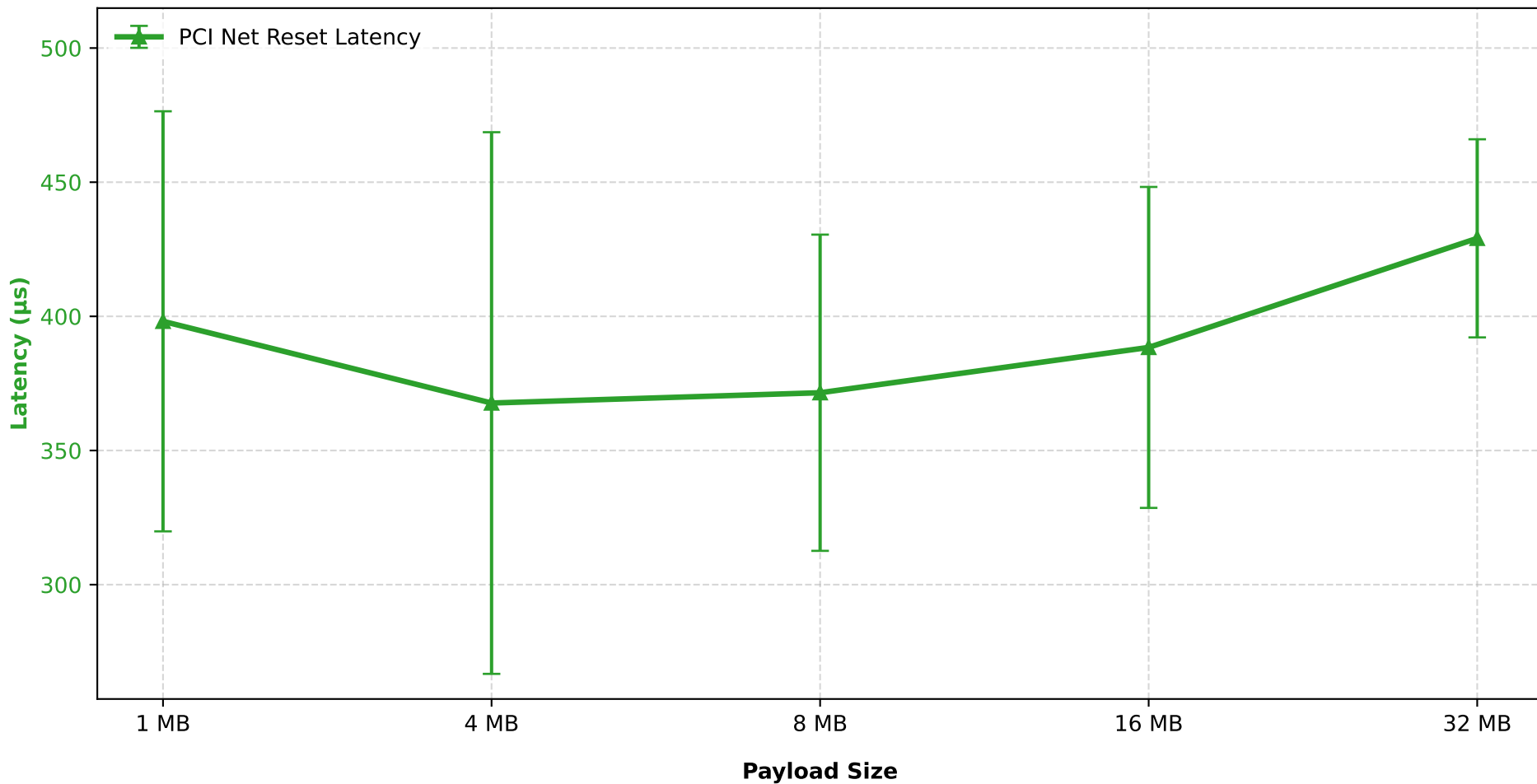
PCI Net Reset Latency vs. Payload Size
