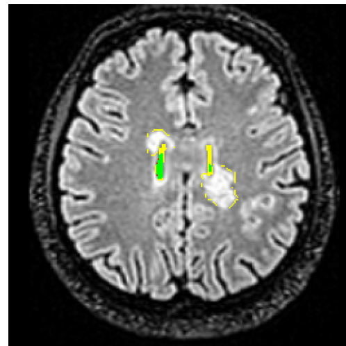
Ventricles Performance
