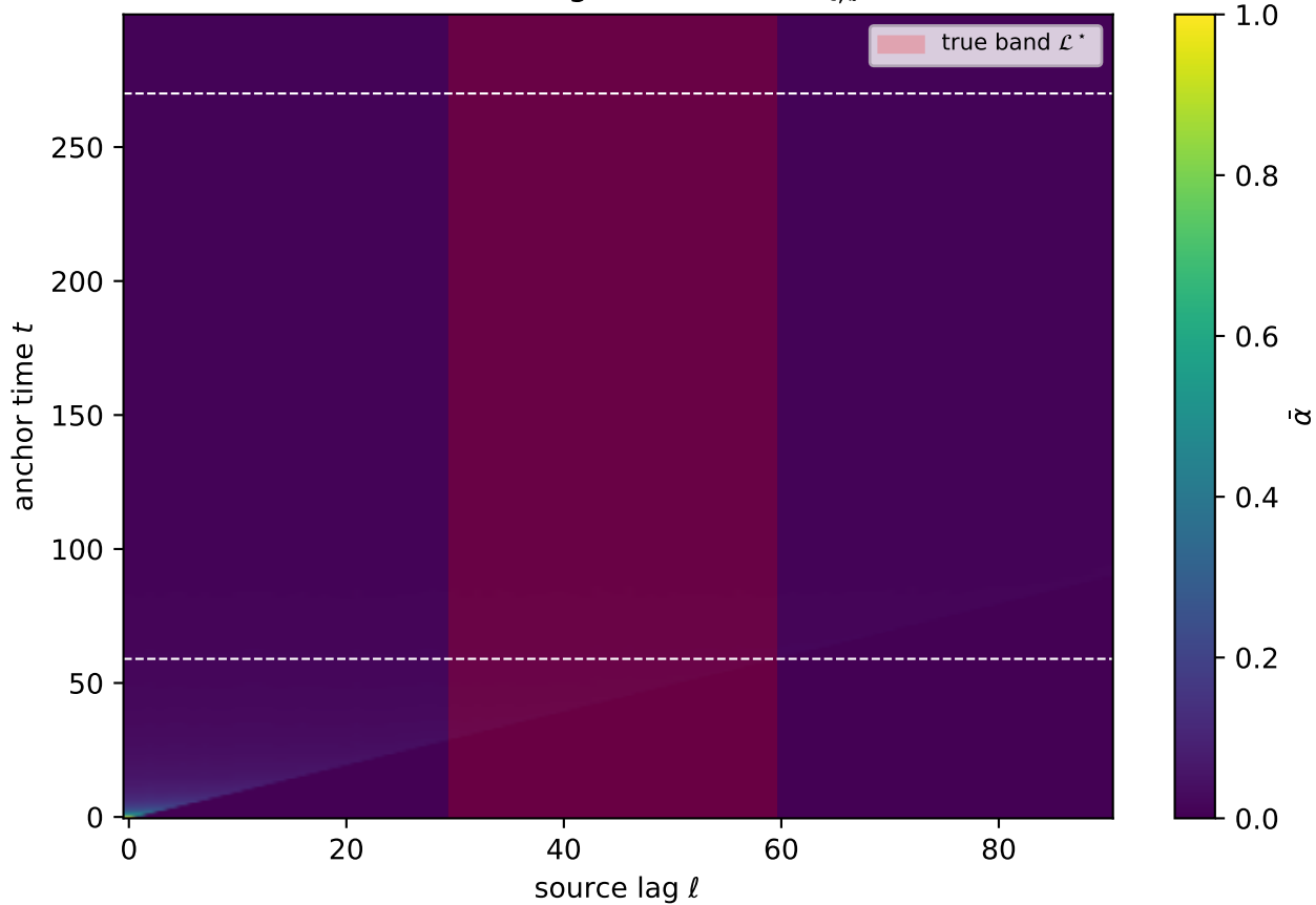
head-averaged attention \bar{\alpha}_{t,\ell}
