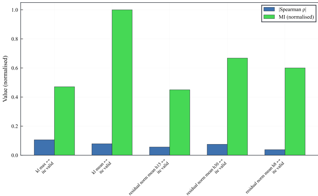
Mutual Information vs Spearman Correlation
