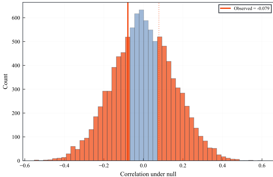
Permutation Test: kl_mean vs ite_valid ( p = 0.6143 )
