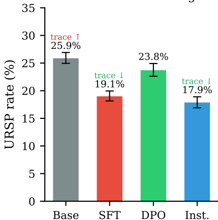
Unfaithful reasoning
