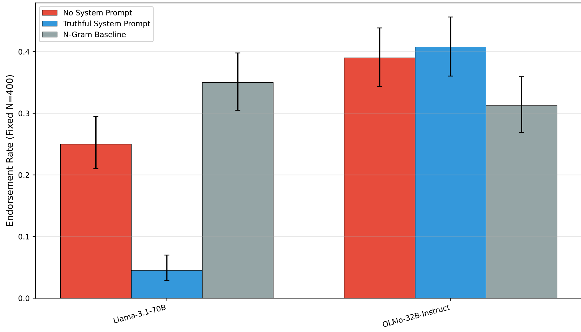
System Prompt Efficacy vs. Syntactic Pressure (T=0.0)
