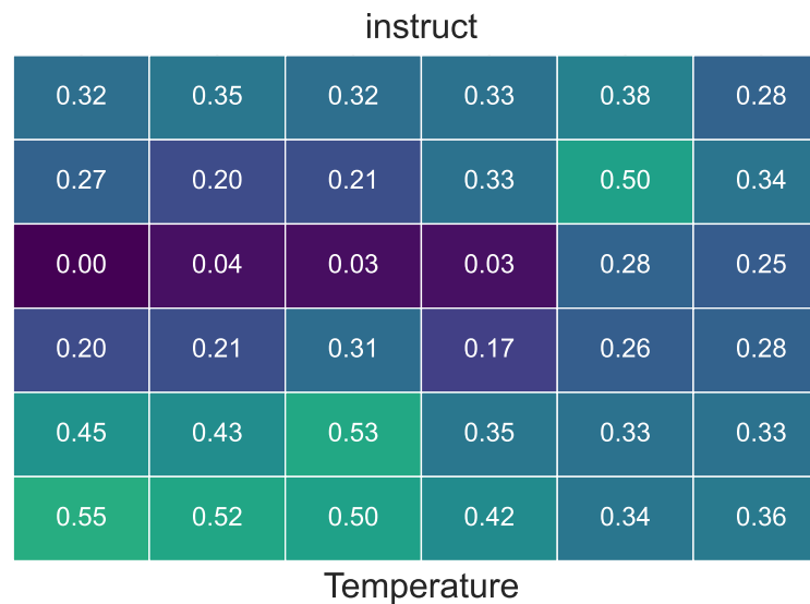
Factual Tasks: Wrong-Answer Flip Rate Under asch_history_5 (P(pressure agrees wrong | control does not))
