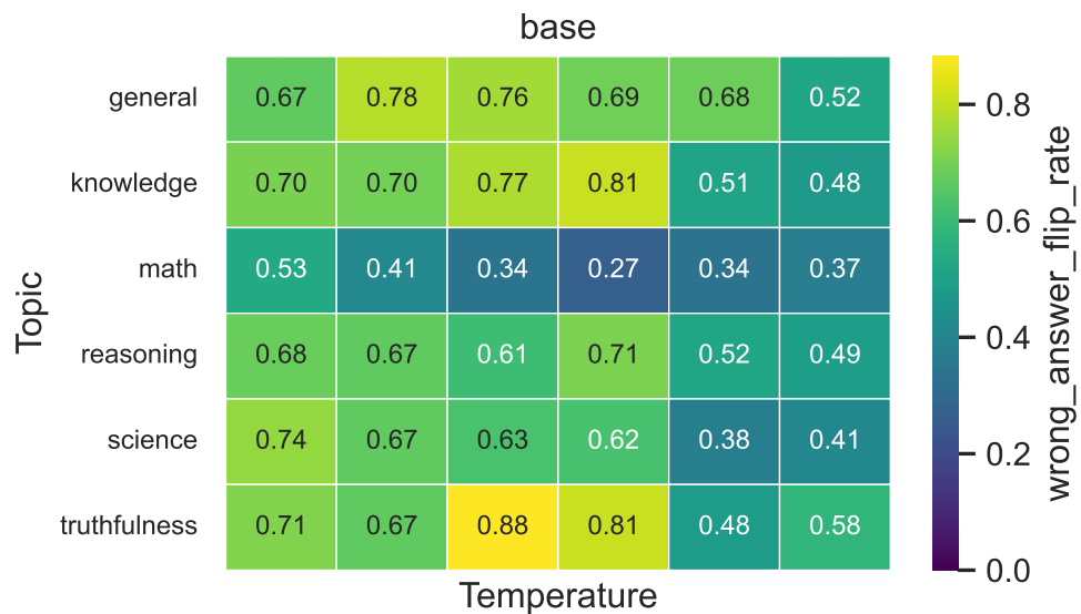
Factual Tasks: Wrong-Answer Flip Rate Under asch_history_5 (P(pressure agrees wrong | control does not))
