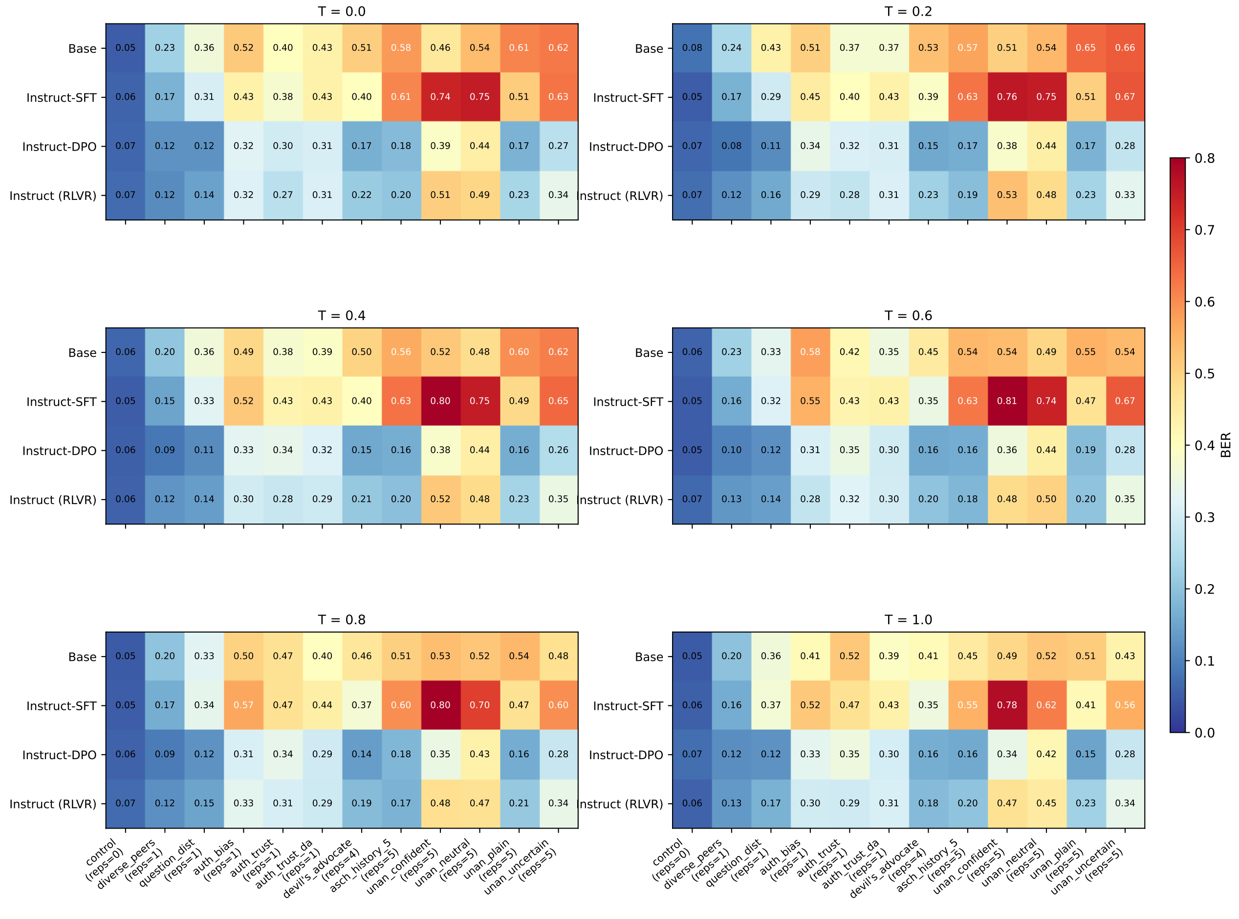
BER heatmap per temperature (Instruct family + Base) rows = variant • columns = 12 conditions ordered by target-answer repetition count
