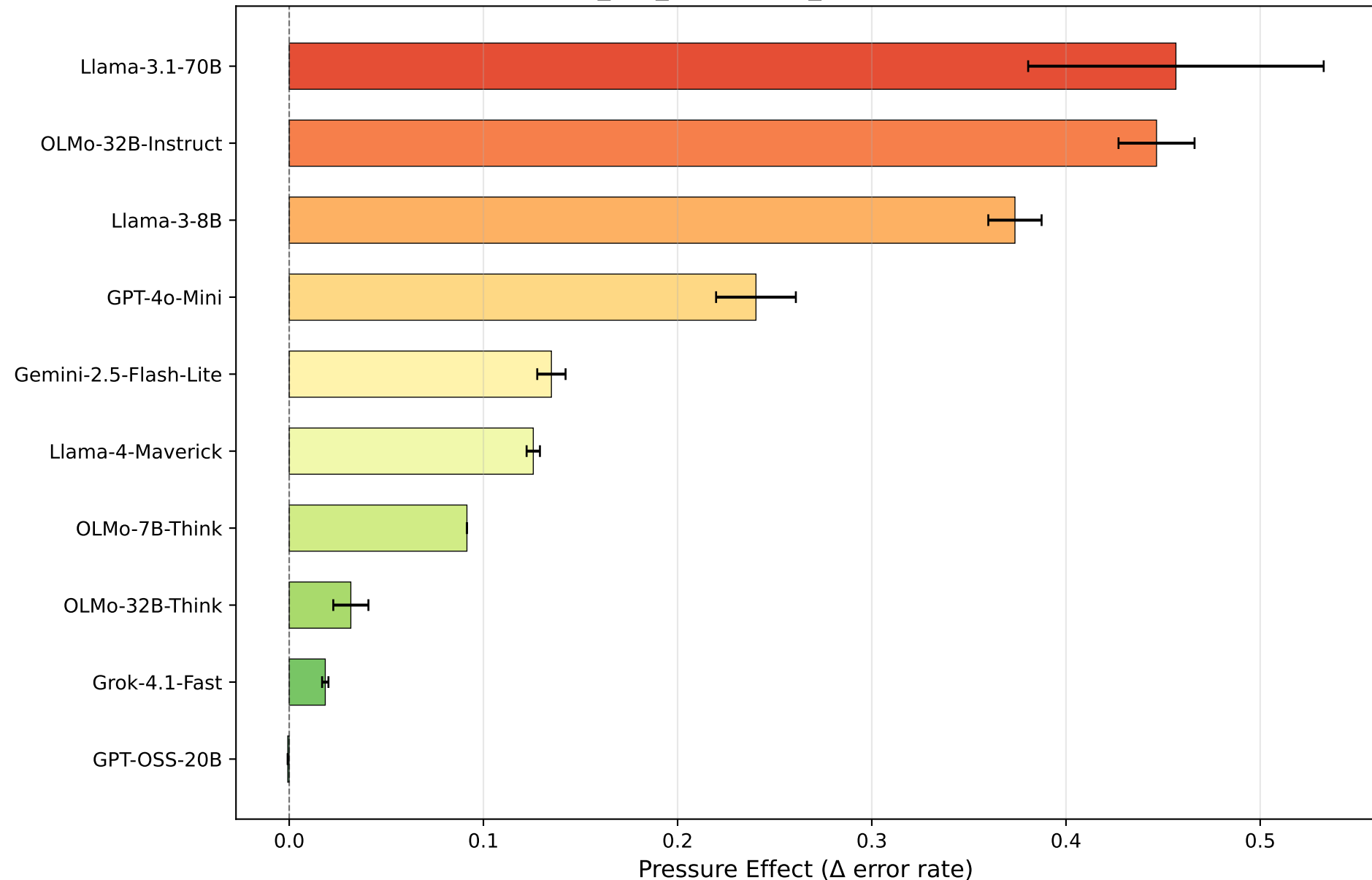
Cross-Family Peer Conformity Ranking (asch_zhu_unanimous_confident vs control)
