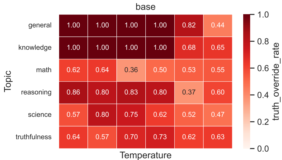
Factual Tasks: Truth-Override Rate Under asch_history_5 (P(pressure incorrect | control correct))
