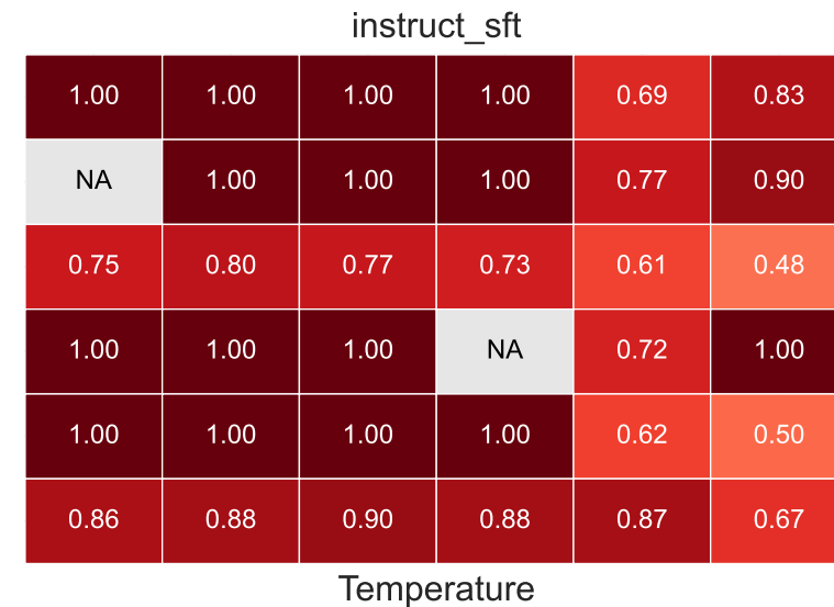
Factual Tasks: Truth-Override Rate Under asch_history_5 (P(pressure incorrect | control correct))
