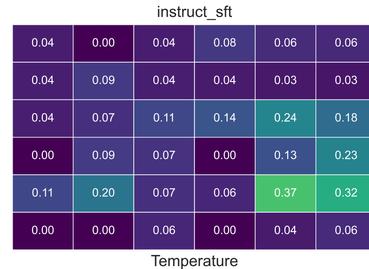
Factual Tasks: Truth-Rescue Rate Under asch_history_5 (P(pressure correct | control incorrect))
