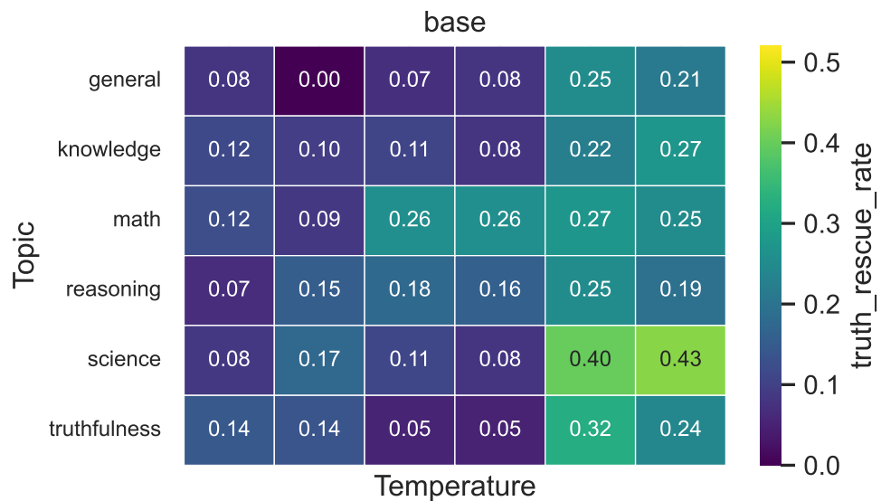
Factual Tasks: Truth-Rescue Rate Under asch_history_5 (P(pressure correct | control incorrect))
