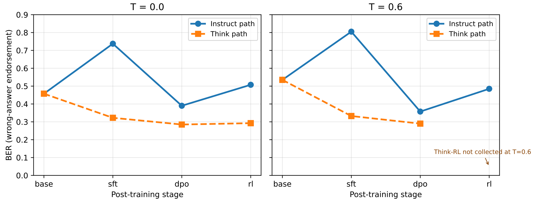
Post-training stage effects on unanimous-confident pressure (7B OLMo)
