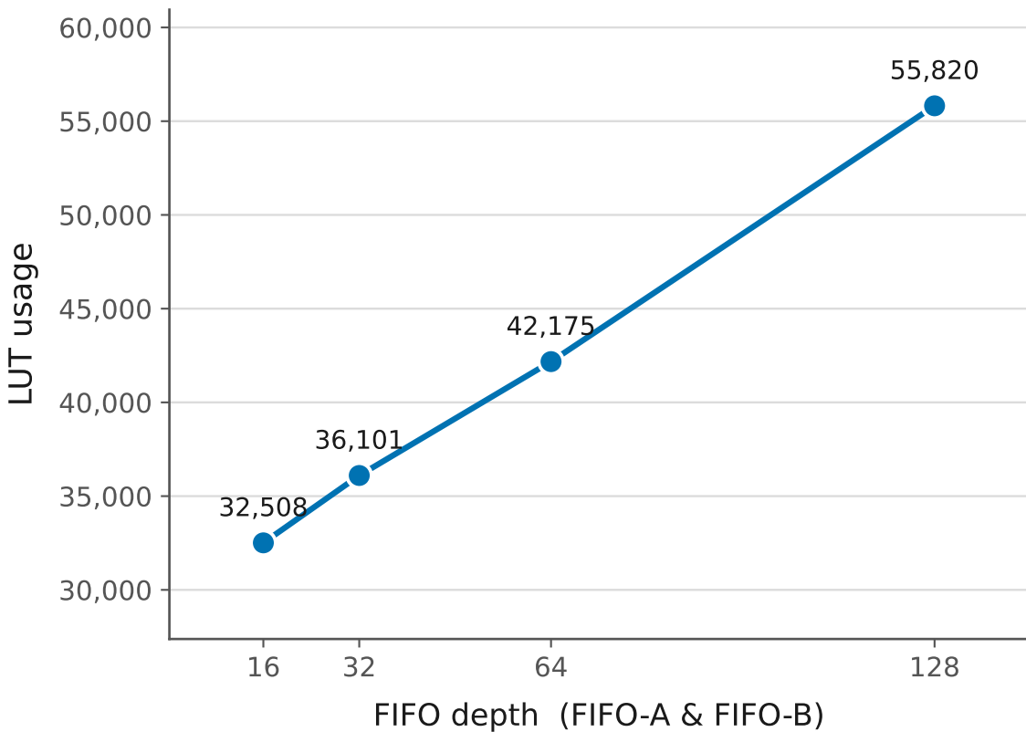
LUT usage vs FIFO_D
