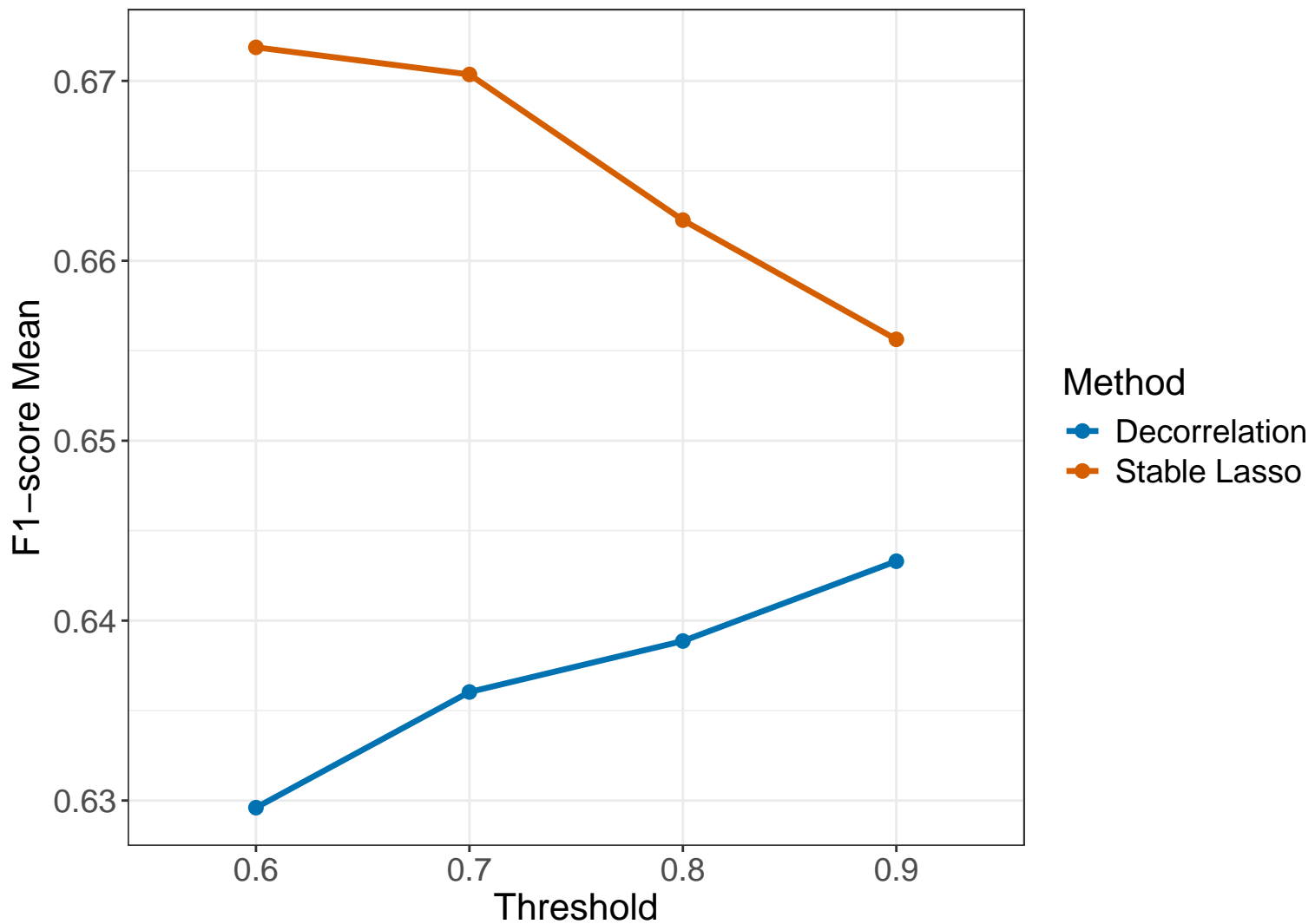
F1-score Comparison
