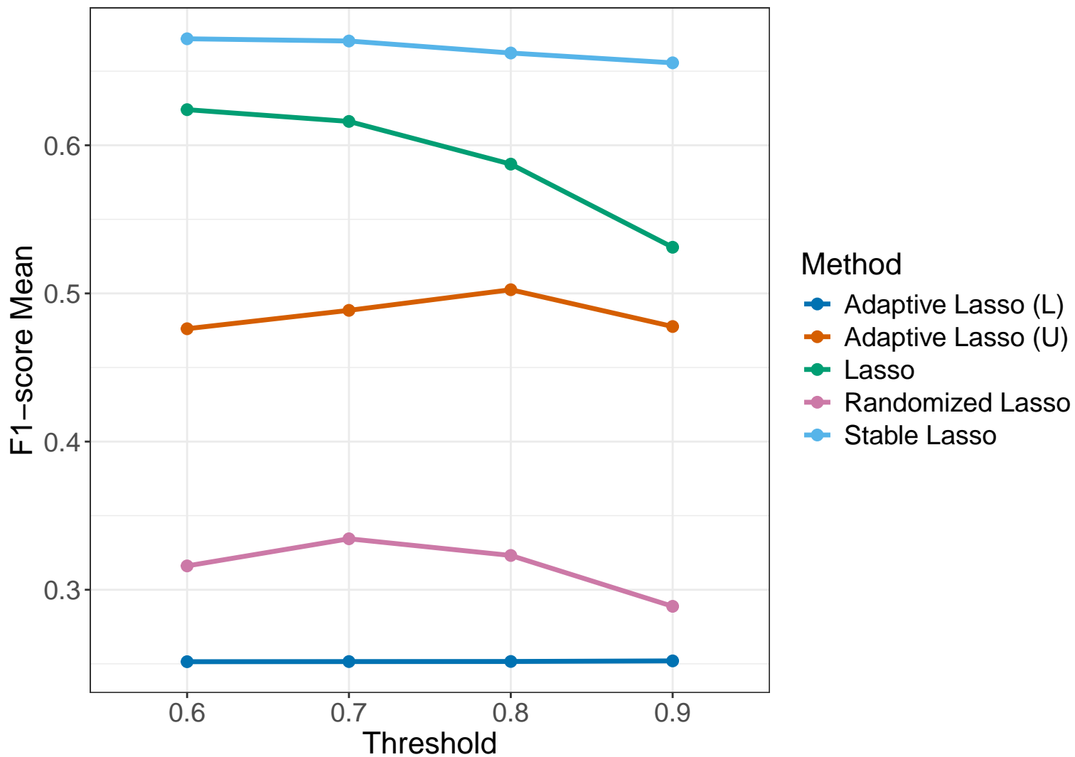
F1-score Comparison
