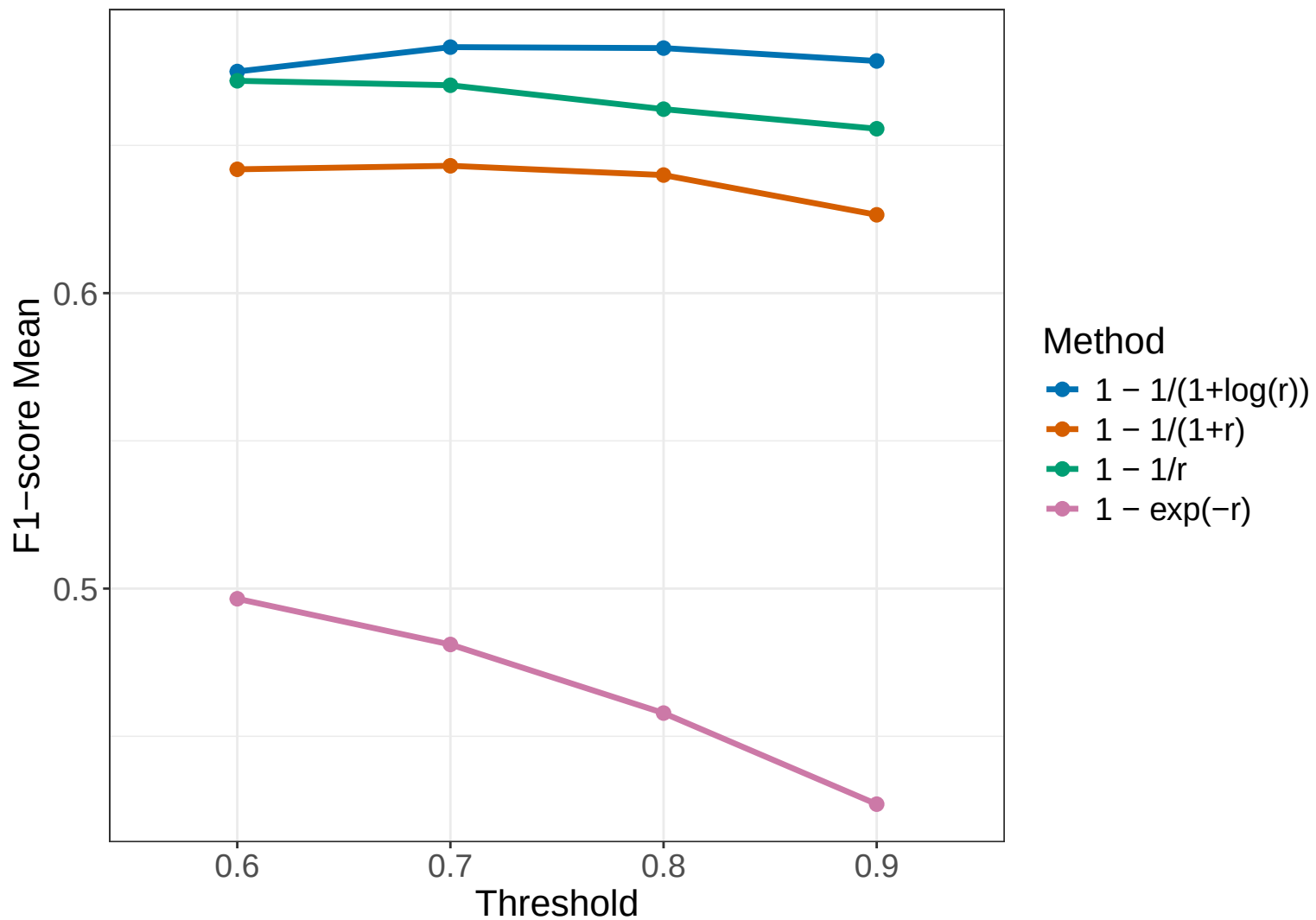
F1-score Comparison
