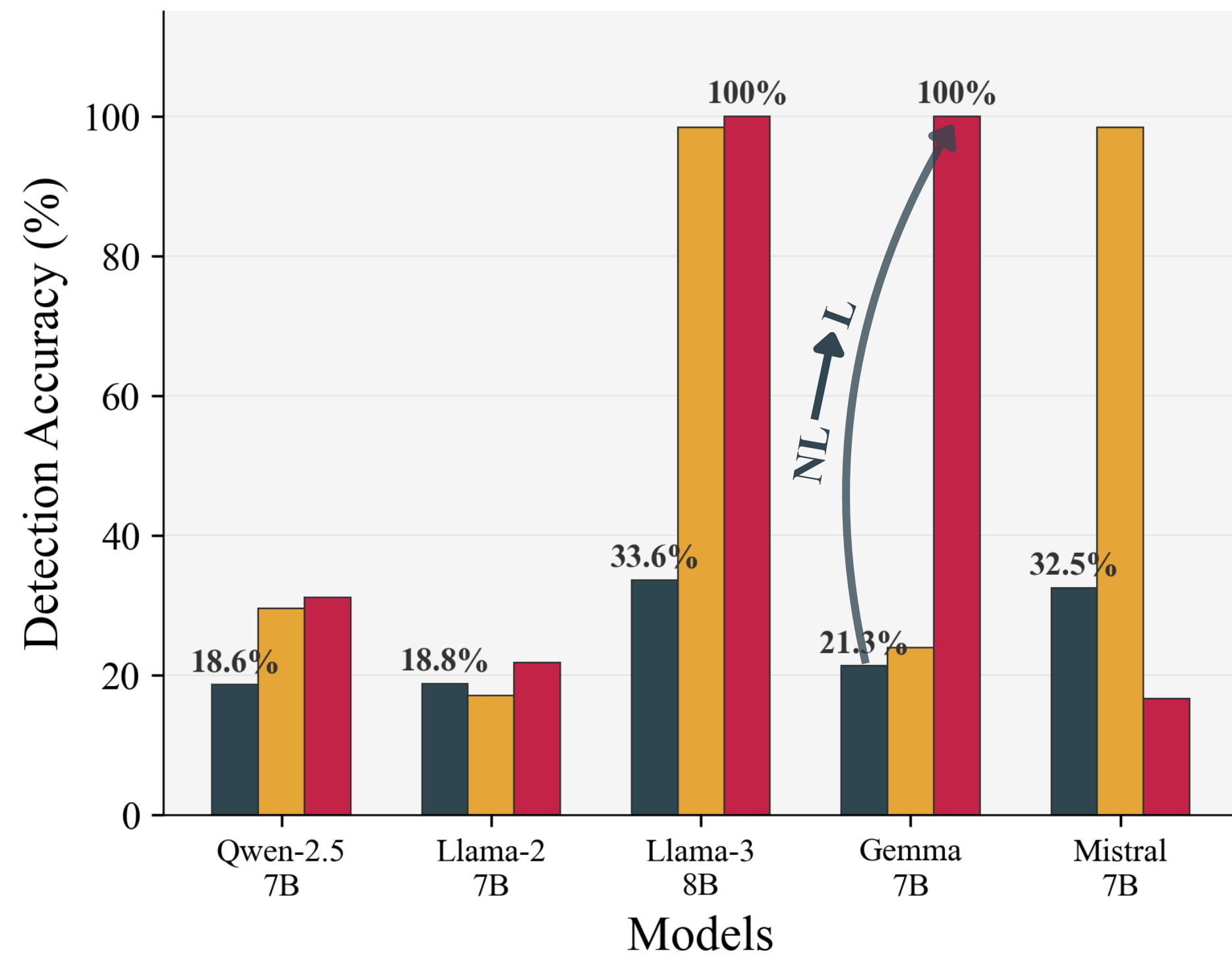
(a) PCA Detector (Linear Subspace)
