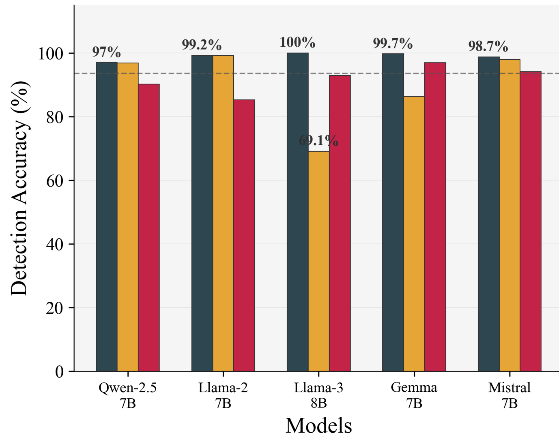
(b) Autoencoder Detector (Non-linear Manifold)
