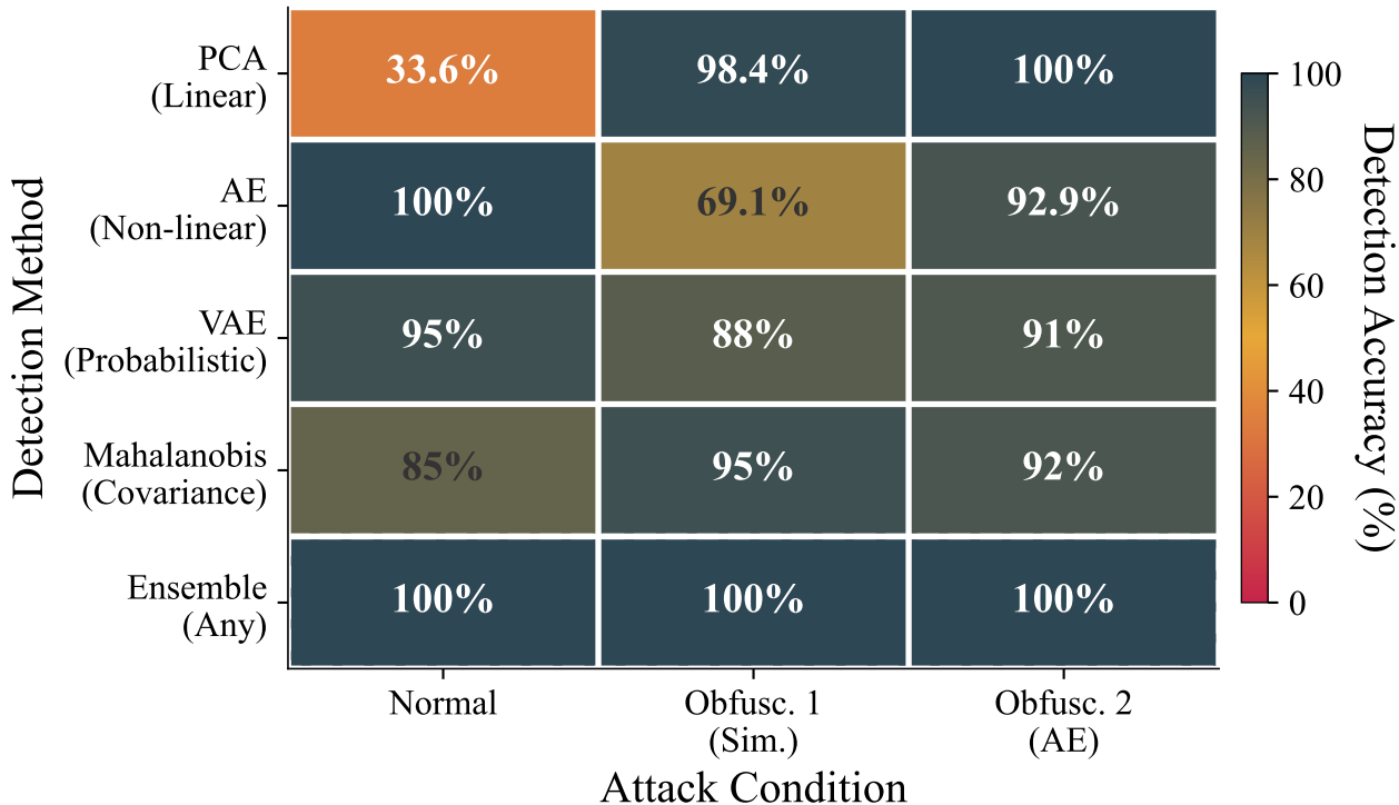
Detector Performance Across Attack Conditions (Llama-3-8B)
