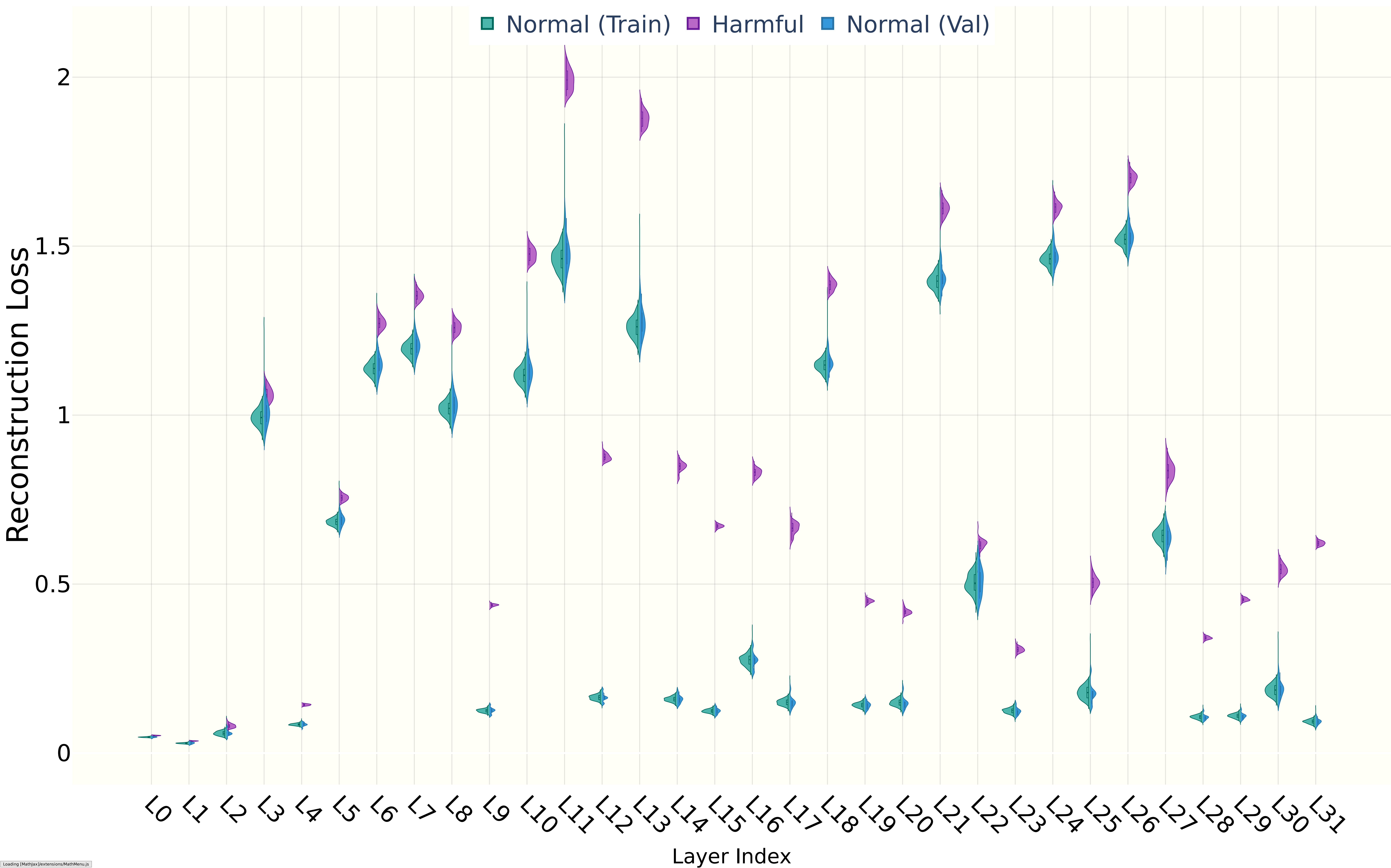
Llama-2-7B-chat-hf Loss Distribution Across All Layers (AE)
