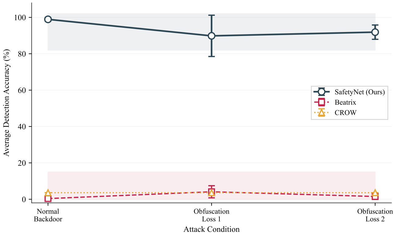
SafetyNet Robustness Under Adaptive Attacks
