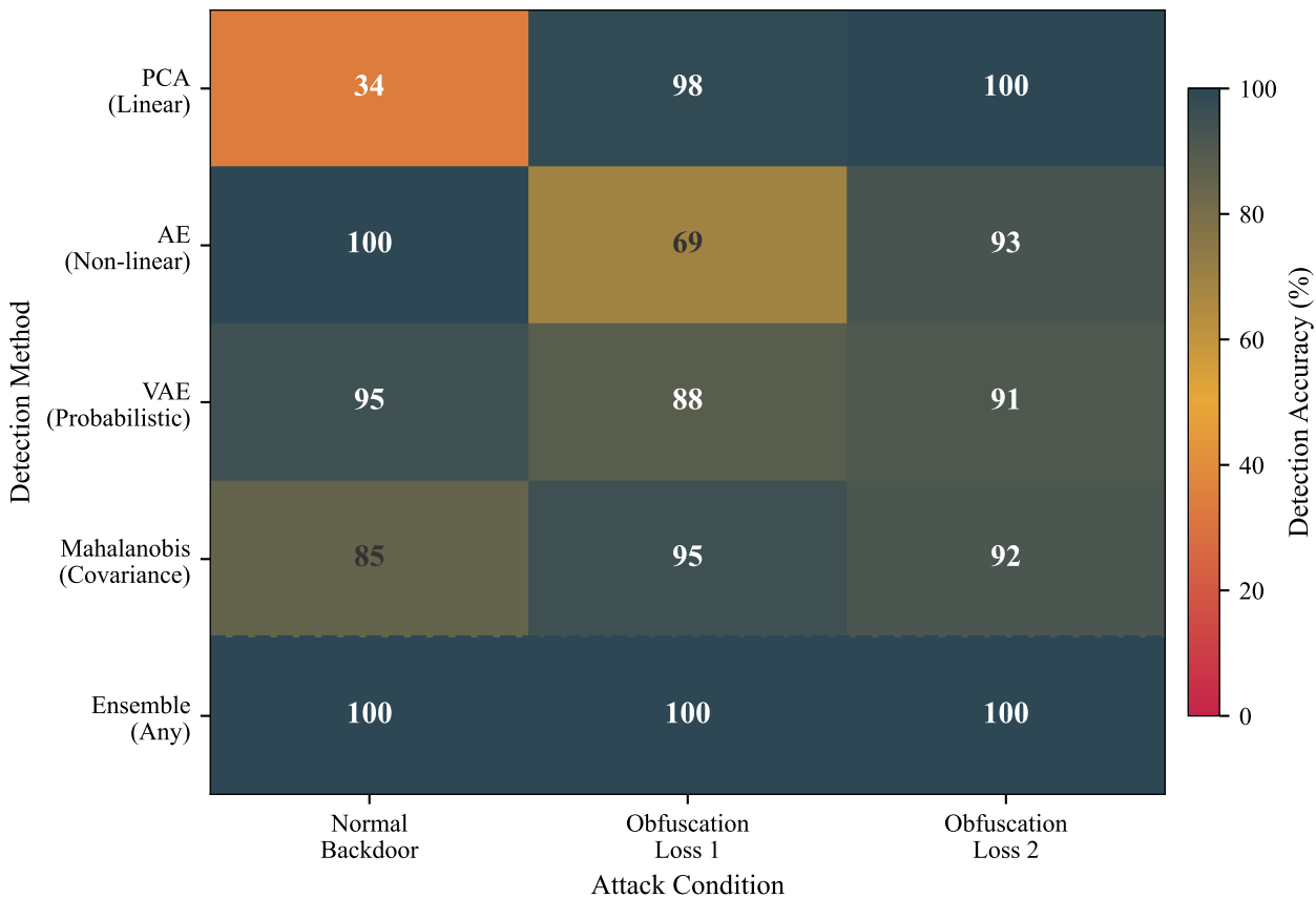
Detector Performance Across Attack Conditions (Llama-3-8B)
