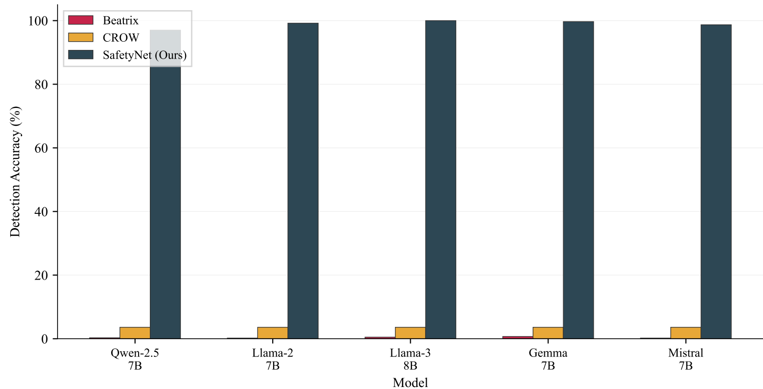
SafetyNet vs Baselines (MAD Benchmark)
