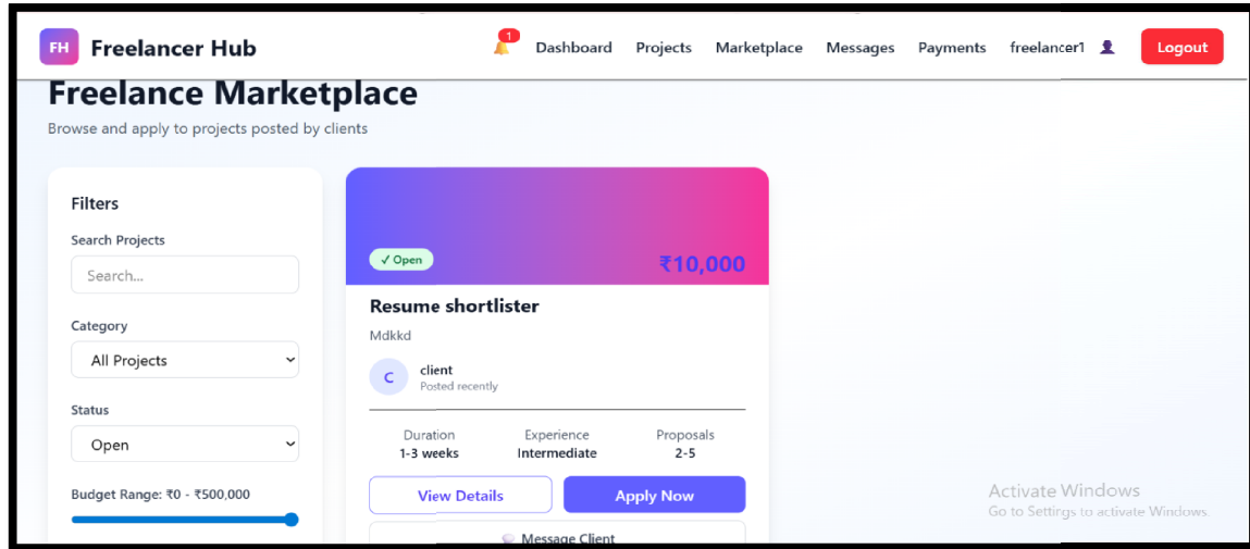
Figure 5: Freelance Marketplace
