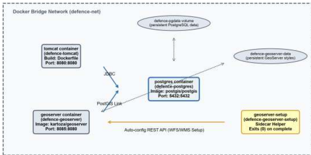
Figure 4.7: Dockerized Multi-Container Network & Volumes Topology Diagram
