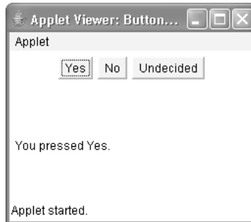
FIGURE 24-1 Sample output from the ButtonDemo applet
