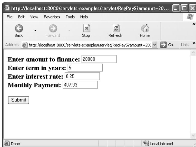
FIGURE 32-7 The RegPayS servlet in action
