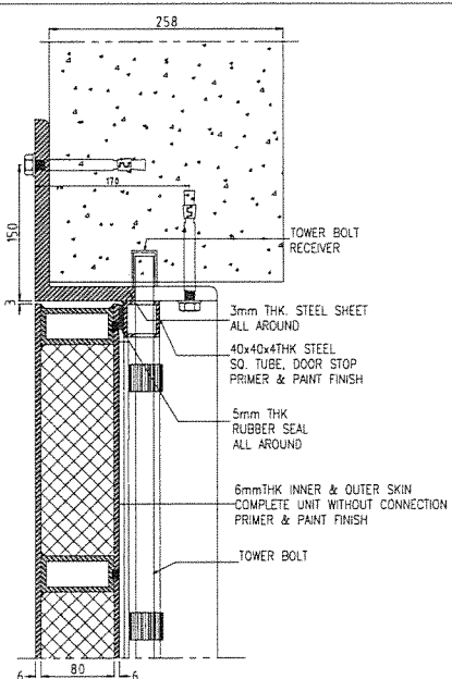
TOP FIXING DETAILS SCALE: 1:3
