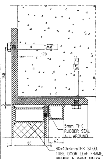
DOORS ARE AIR TIGHT BECAUSE OF WEATHER STRIPPING
