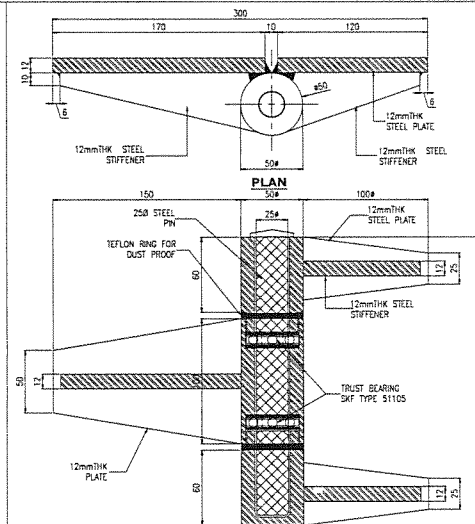
DETAIL @ WELDED STEEL BARREL HINGE SCALE: 1:2
