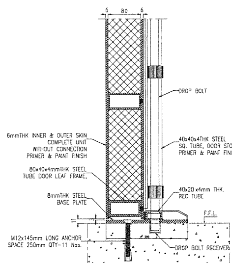
BOTTOM FIXING DETAILS SCALE: 1:2
